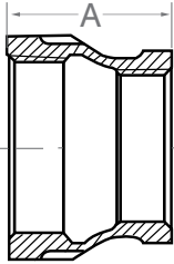
UL/FM: 1/2" to 1 1/2"
